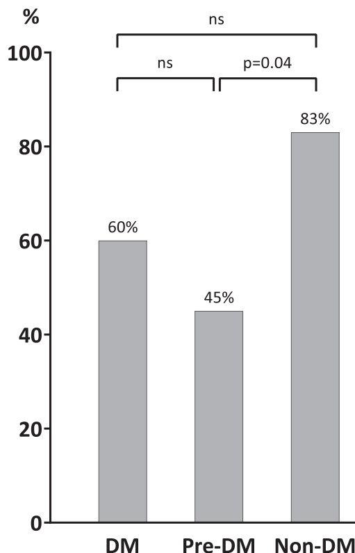
Figure 2. Rate of patients receiving a transplanted islet mass of over 2000 IEQ/kg. A similar proportion of patients received a clinically relevant islet mass of over 2000 IEQ/kg during the transplantation in the DM and non-DM groups: 60% (3/5) and 83% (15/18) (83.3%) (NS), respectively. Of note, significantly fewer patients received such an islet mass in the pre-DM group (45% [5/11]) as compared to the non-DM group (P=.04). DM = diabetes mellitus, IEQ = islet equivalents, NS = not significant.
