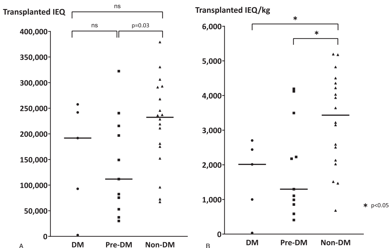
Figure 1. Islet mass retrieved and transplanted from diabetic, pre-diabetic, and non-diabetic patients. (A) Islet mass expressed in islet IEQ isolated and transplanted in the DM group did not differ significantly from that in the pre-DM and non-DM groups (NS). However, islet mass in the pre-DM group was significantly lower than that in the non-DM group ( P = .03 ). (B) Islet mass transplanted per patient body weight in kilograms (IEQ/kg) did not differ significantly between the DM and pre-DM groups. However, it was significantly higher in the non-DM group than both other groups ( P < .05 ). DM = diabetes mellitus, IEQ = islet equivalents, NS = not significant.
